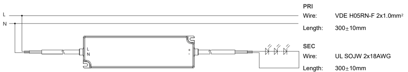
Wiring Diagram
